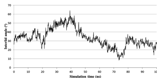
Fig. 6. Inter-lid angle between lid A and lid B of lipMKNK during lid opening movement at 20% acetonitrile. The inter-lid angle was measured based on the angle formed by C \alpha position of Ser19, Asp175, and Phe221.
