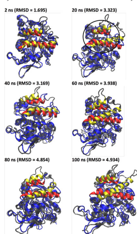
Fig. 5. Snapshot of lid movement for every 20 ns simulation. The initial and final conformation of lid in every 20 ns of the simulation were represented by red and yellow ribbon. The other part of the protein were presented as gray and blue ribbons for the initial conformation and every 20 ns of simulation. All structures were generated in new cartoon model by VMD. Circle was point out of lids; ns = nano second
