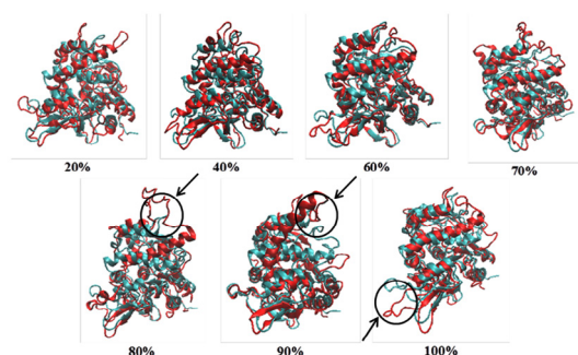
Fig. 2. Superimpose between lipMNK structure after 100 ns MD simulation in various acetonitrile concentrations (red) and structure of lipMNK at 0% acetonitrile (blue). The unfolded segment due to the presence of acetonitrile was pointed by arrow. All protein structures were generated in cartoon model by VMD
