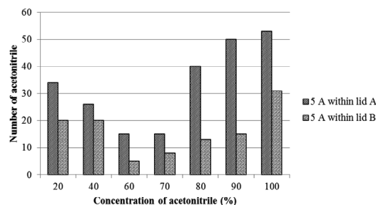
Fig. 4. The number of acetonitrile molecules within 5 Å distance from the lid segment in different acetonitrile concentrations (%)
