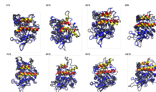
Fig. 3. Snapshot of lid opening movement in various acetonitrile concentrations. Initial lid position was presented in red, while the lid position after 100 ns was depicted in yellow. The other part of the protein was presented as gray and blue ribbons for the initial state and after 100 ns simulation. All structures were generated in new cartoon model by VMD
