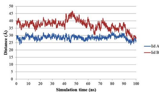
Fig. 8. Dynamic pattern of lid A and lid B in o-lipMNK during closing movement. Blue and red lines represent the respective distance covered by Ser195 (lid A) and Phe221 (lid B) relative to Ala289 (non lid region)
