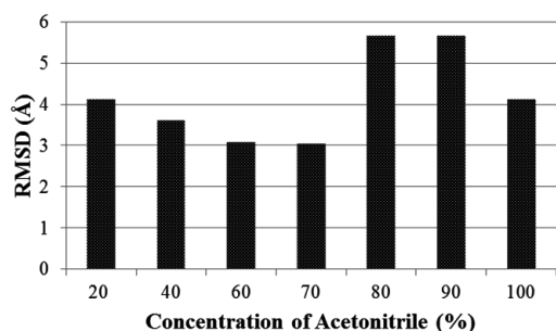
Fig. 1. RMSD of c-lipMNK in various concentration of acetonitrile after 100 ns of MD simulation. RMSD was calculated using c-lipMNK structure in 0% acetonitrile at 100 ns of MD simulation as reference. Å = Angstrom
