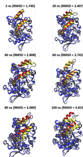
Fig. 7. The snapshot of lid closing movement every 20-ns time interval. Red and yellow helices represent lids at the initial (open) and final conformation at each time interval, respectively. The other parts of protein conformation were represented as blue and gray for the respective initial and at the time interval.
